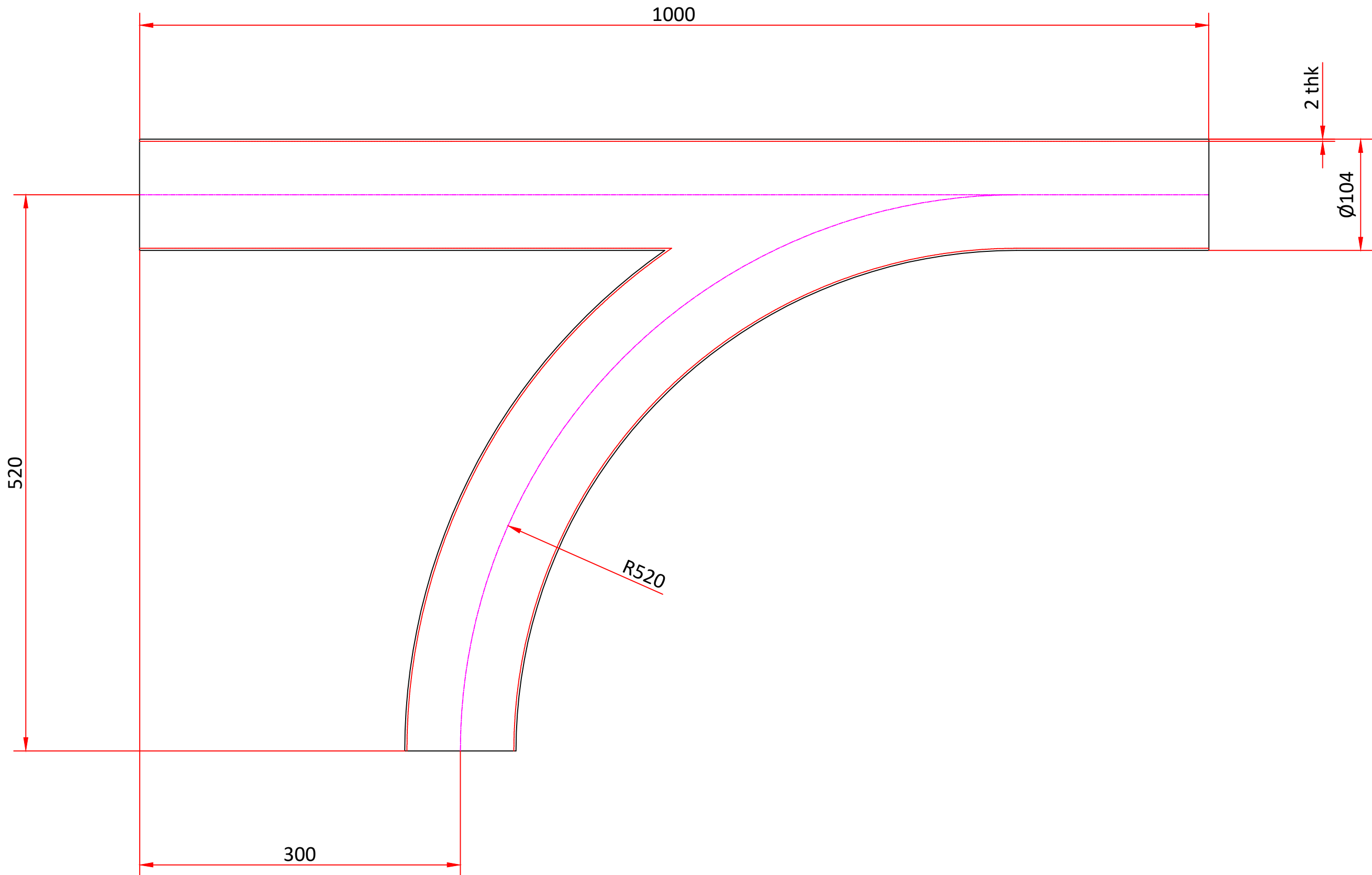
4" SWEPT TEE
